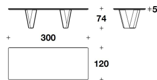
VTB (27E) TAVOLO RETTANGOLARE / RECTAGULAR TABLE 300x120x74H. - THK.5cm 118x47 1/3x29H. - THK.1 15/16"
