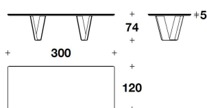
VTB (27M) MARBLE : TAVOLO RETTANGOLARE / RECTAGULAR TABLE 300x120x74H. - THK.5 cm 118x47 1/3x29H. - THK.1 15/16 "
