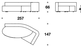
DRAWING: RIGHT ELEMENT
