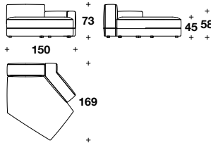
DRAWING: RIGHT ELEMENT
