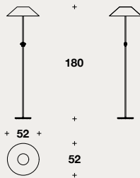
HIGH STANDING LAMP: VMP (02)
